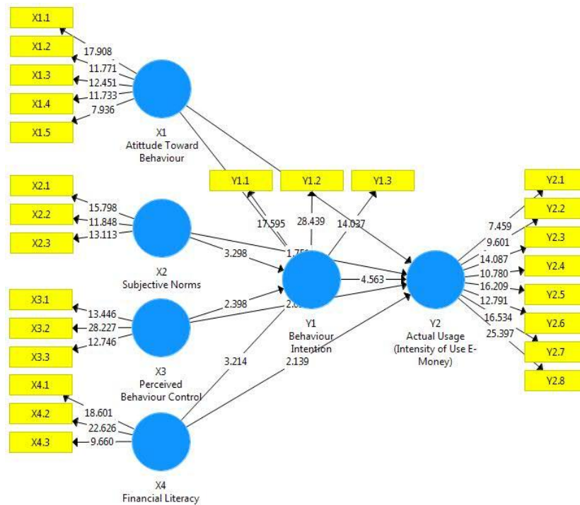
Figure 2. Schematic Bootstrapping of PLS Model
